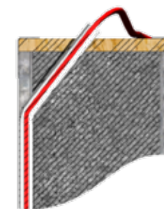
Drill hole through top tray and EPS to thread conduit through.
