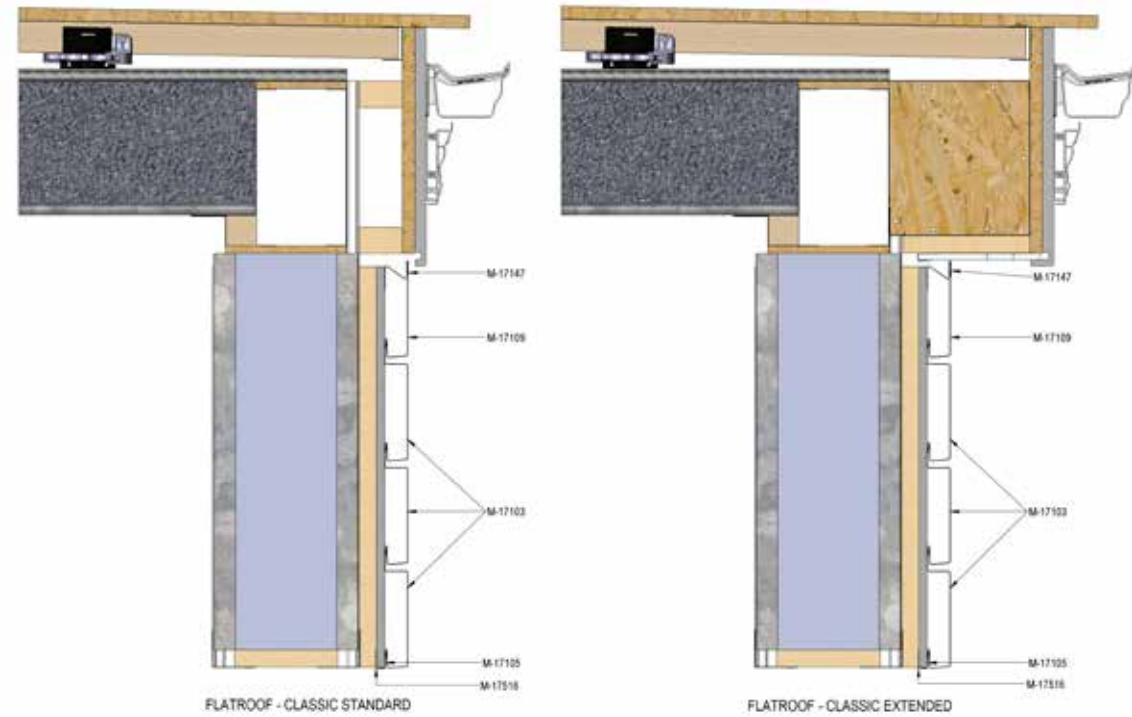
Flatroof classic with Facade
