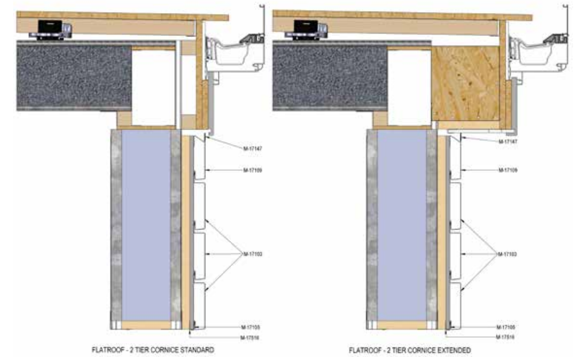
Flatroof 2 tier with facade
