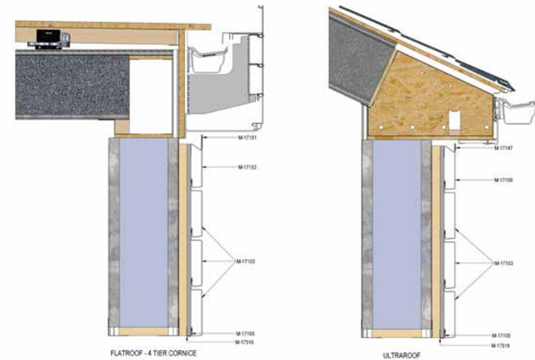
4 tier and ultrarroof with facade
